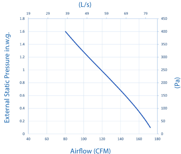
E130-HRX-N Ventilation Performance
