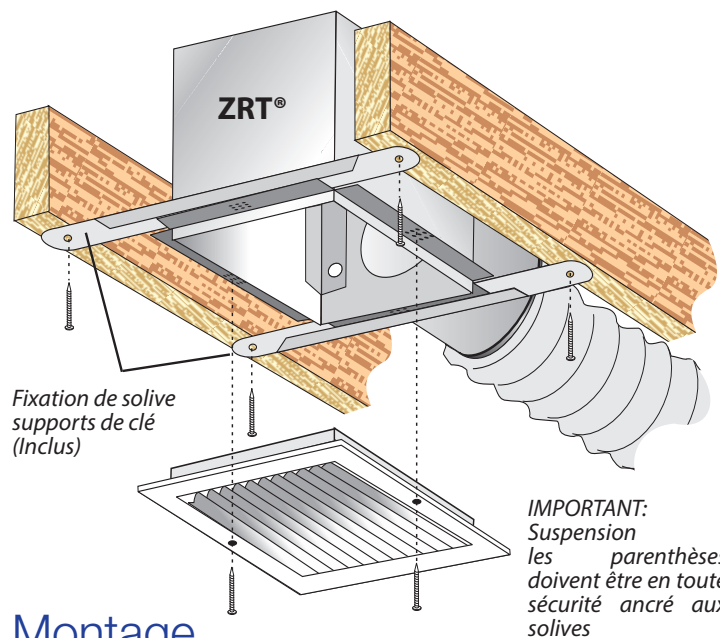
FIGURE 1 - MONTAGE
