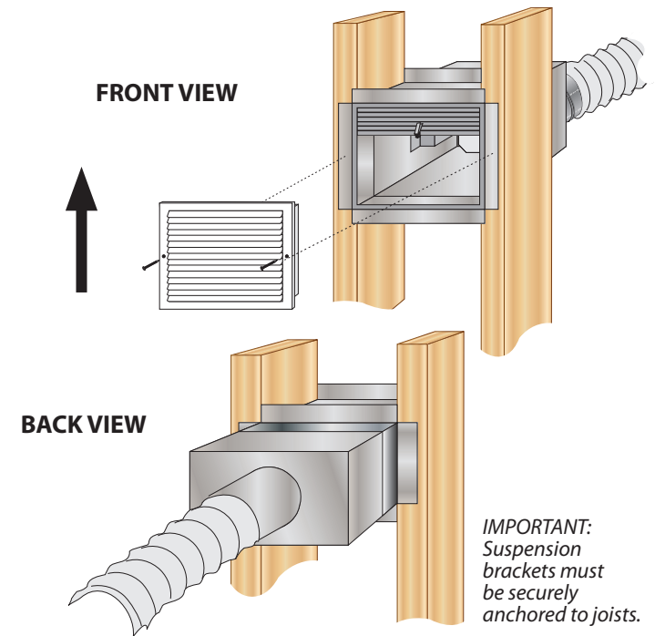
FIGURE 1 - MOUNTING
