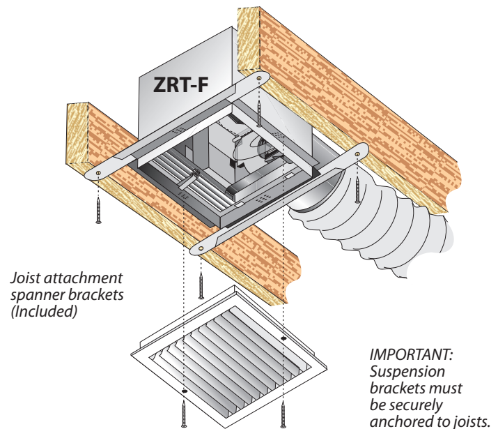
FIGURE 1 - MOUNTING
