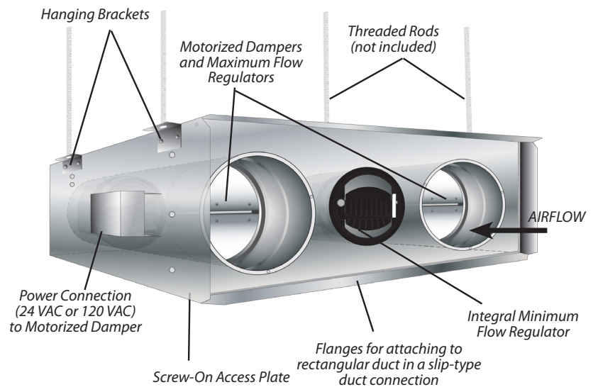
FIGURE 1 - MOUNTING
