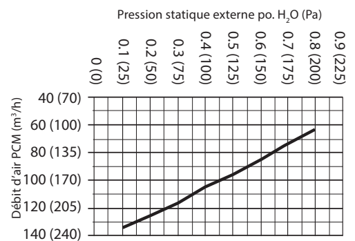
E150-TRG Performance de ventilation
