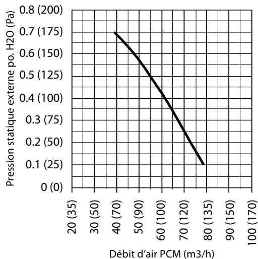
H80-HR-N Performance de ventilation
