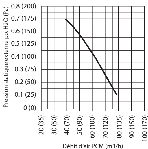
H80-HF-N Performance de ventilation
